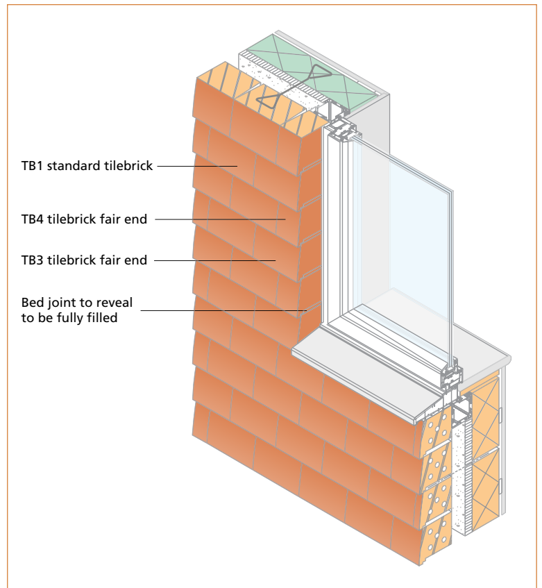
Isometric of window jamb detail
