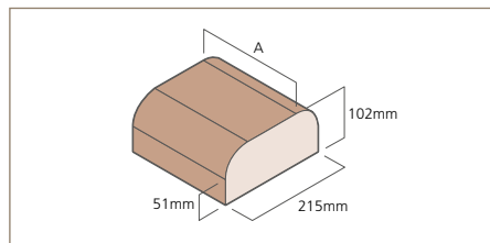
FB22 Double Bullnose
