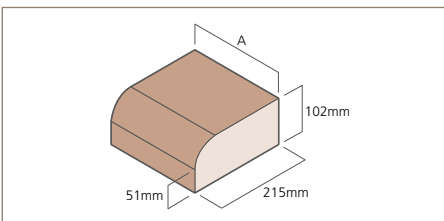
FB12 Single Bullnose
