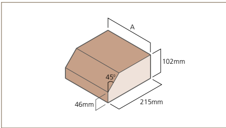
FA51 Single Cant
