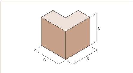
FC1 External 90° Corner
