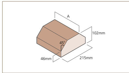
FA61 Double Cant
