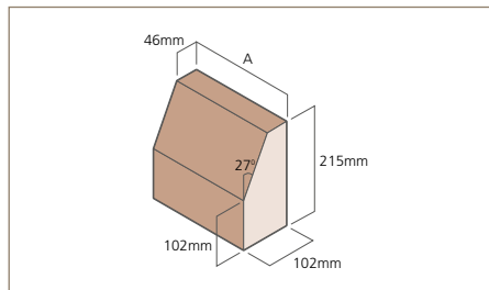
FBD2 Sill Brick
