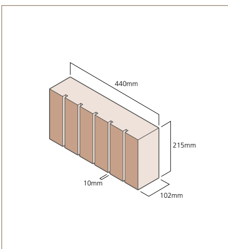
SOLDIER Standard Soldier Unit
