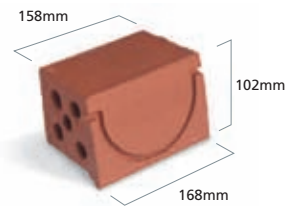
Unit TB 16 club Tilebrick™
