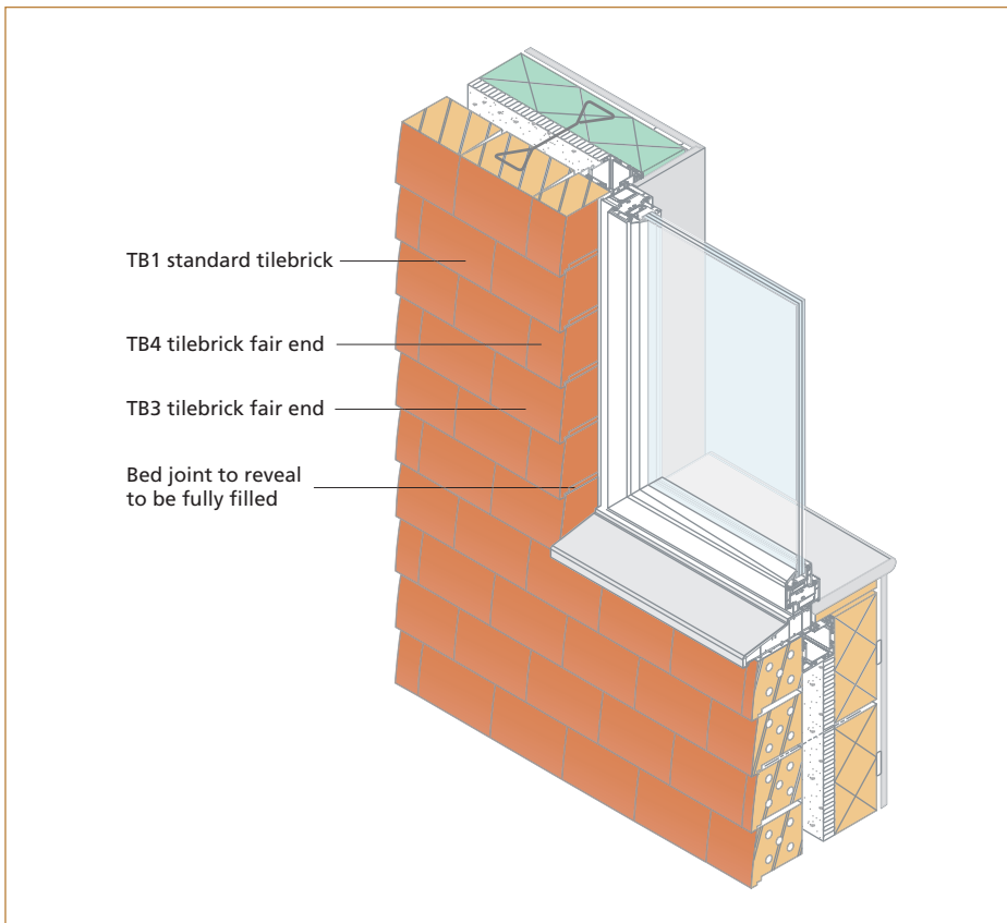
Isometric of window jamb detail
