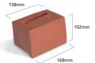
Unit TB 3 fair end 1 Tilebrick™
