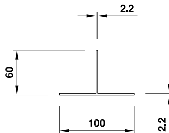
Plan on Rail (Scale 1:5)
