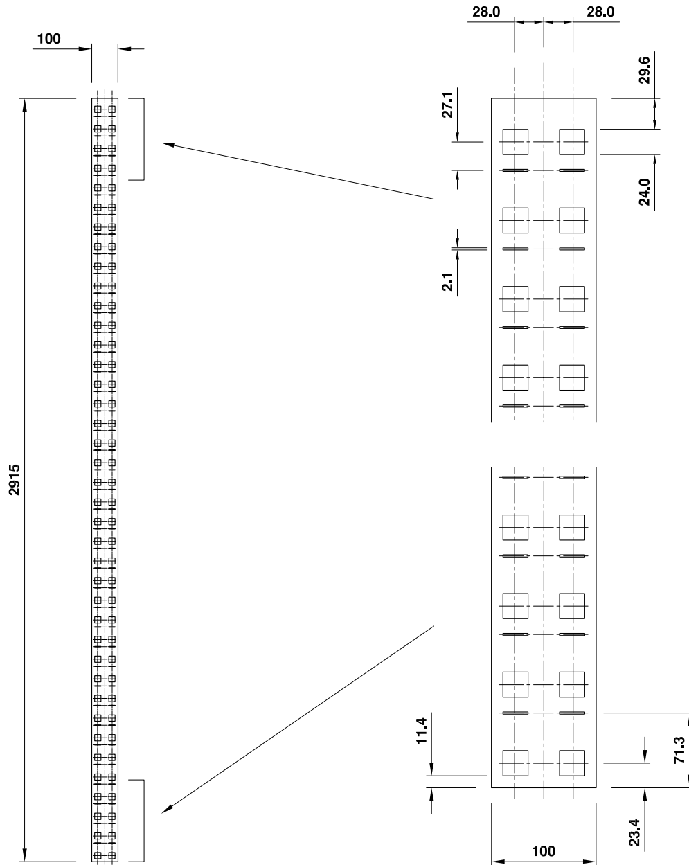
Elevation on Rail (Scale 1:20)
